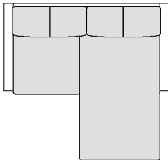
C Sofa 158 + C Ottoman 063 W158 . D150 . 5. H75 . SH38
