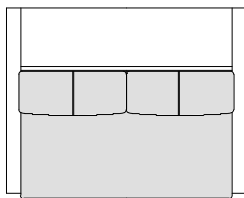
C High Sofa 158 W158. D87.5. H75. SH38
